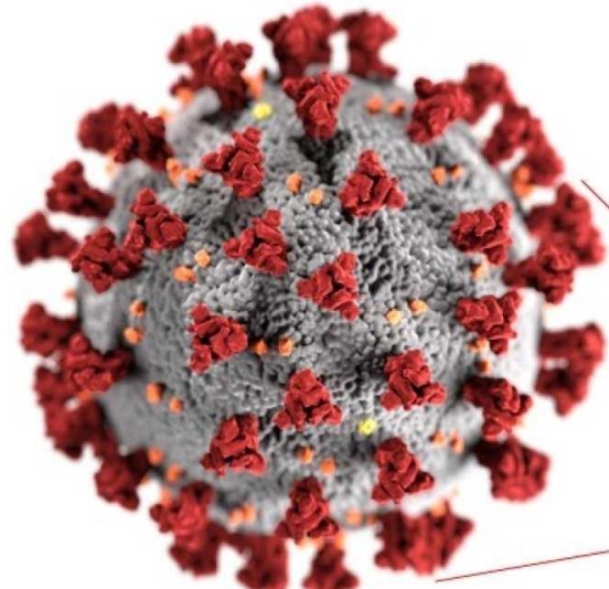
Coronavirus-containing aerosols
